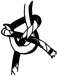
Modern Midshipman Hitch
