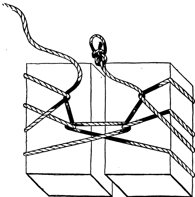
Fig. 7. The hitch is now cinched.
